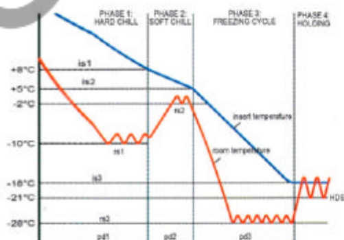
2 CY2: Hard chill + soft chill + freezing + holding
